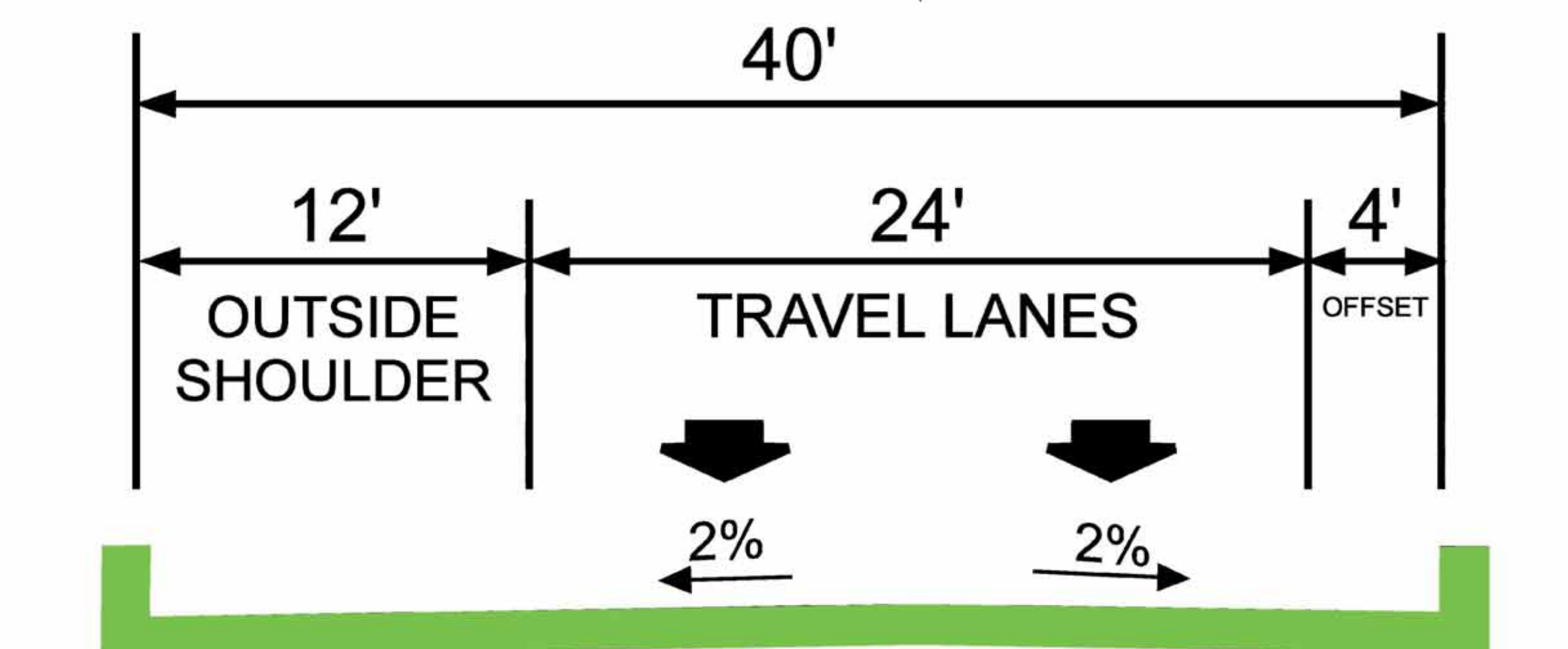
PROPOSED BRIDGE TYPICAL SECTION (2 LANES)
