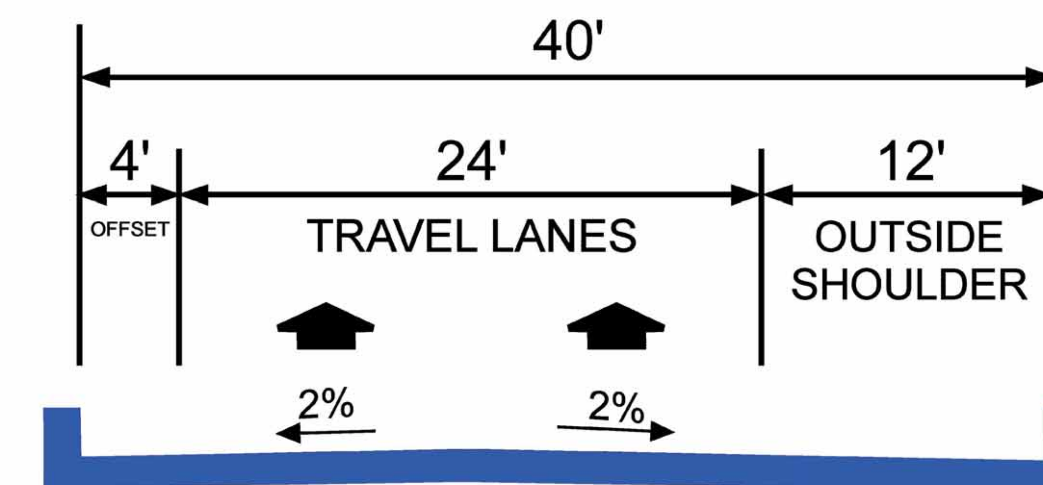
PROPOSED BRIDGE TYPICAL SECTION (2 LANES)
