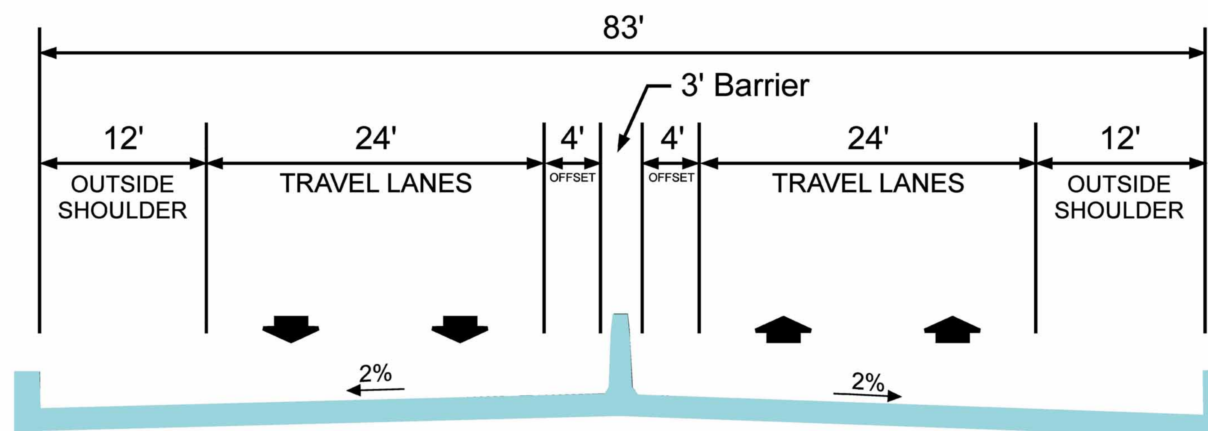
PROPOSED BRIDGE TYPICAL SECTION (4 LANES)
