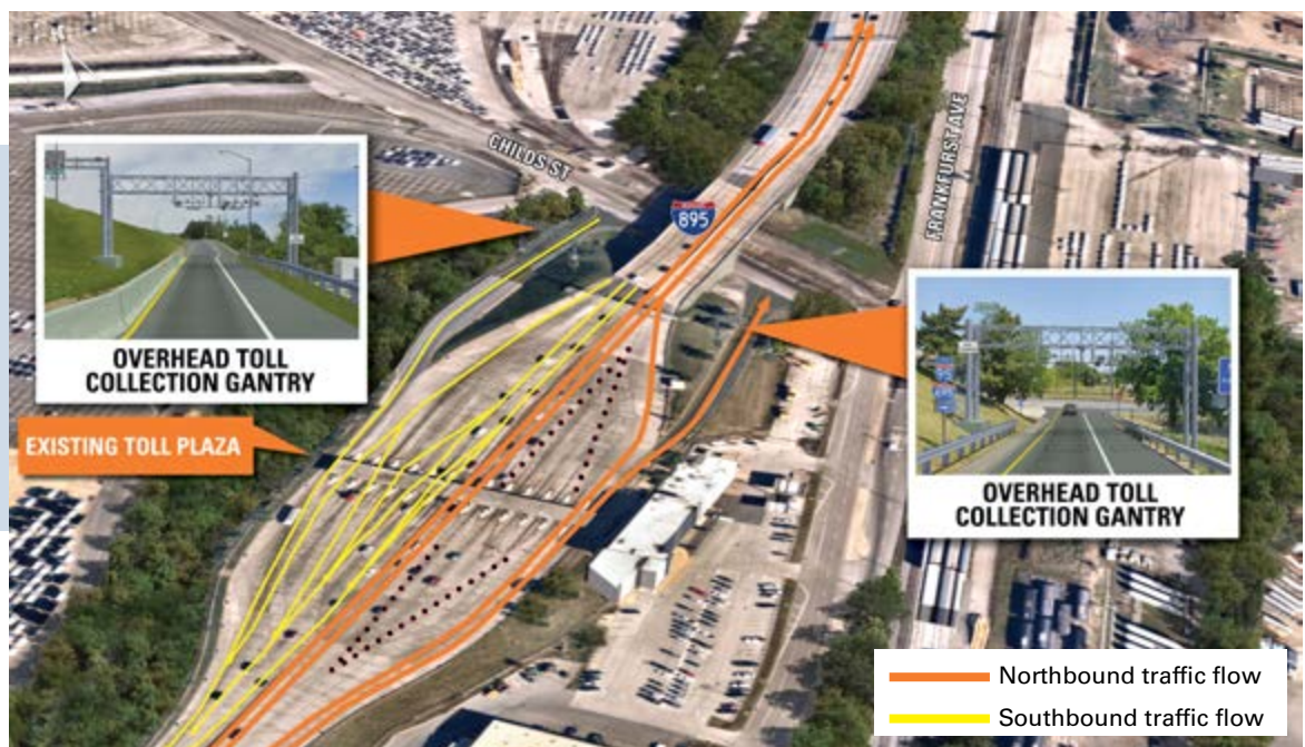
Overhead Toll Collection Gantries - Childs Street Entrance and Exit Ramps
